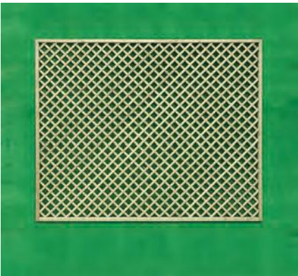
Diamond Lattice
